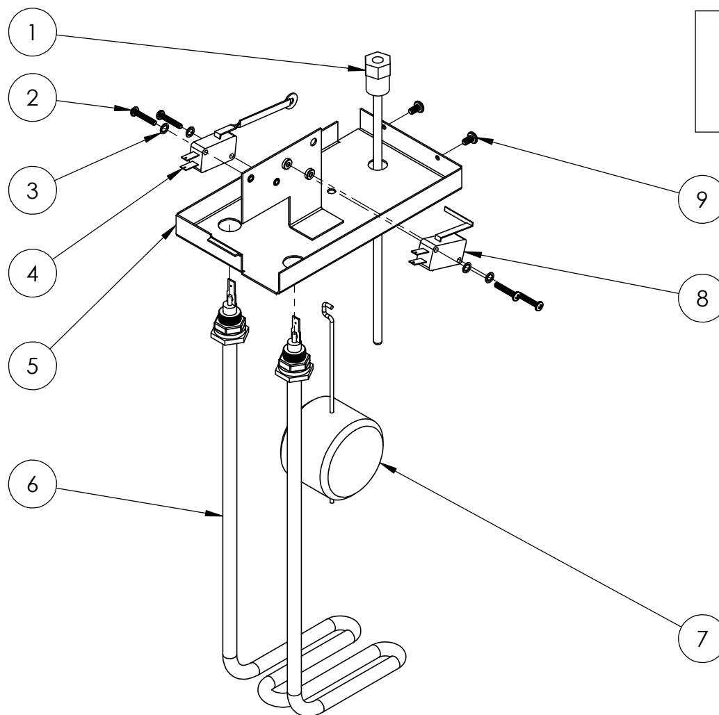
09ASS18 WATER TANK LID ASSY (PROBE) S-A COUV. RESERVOIR COURT (SONDE)
