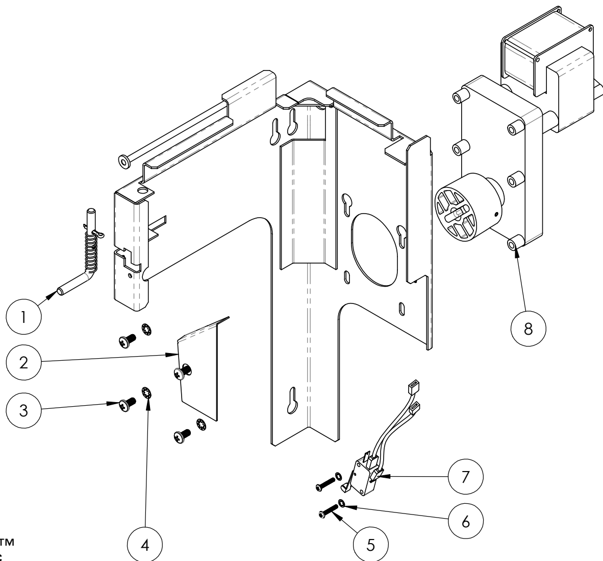
96ASS20P PLATINUM BREWER BRACKET S-A S-A SUPPORT INFUSEUR PLATINUM
