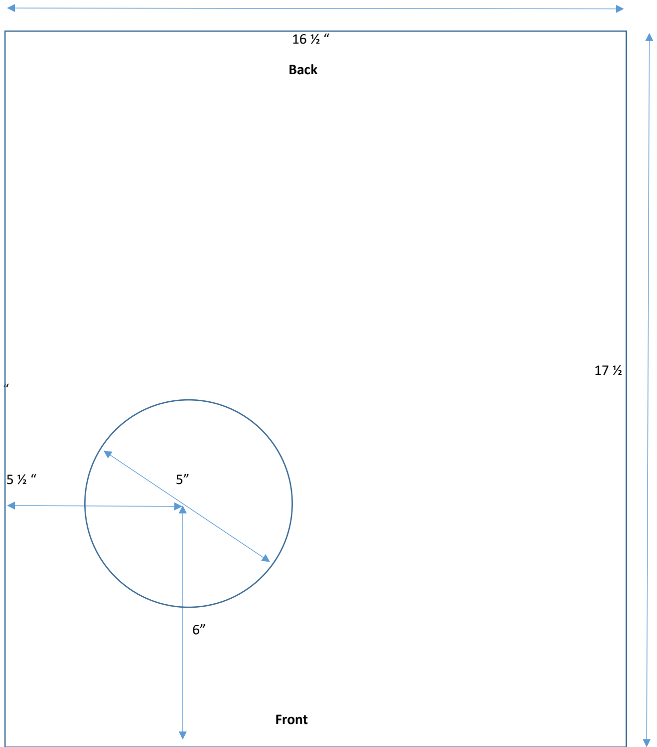
9100 Ground Chute Counter Top Hole Location
